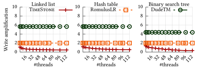
Figure 9. Comparison of write amplification incurred in different DTM systems for a write-intensive workload.
