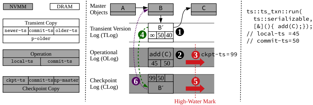
Figure 2. Illustrative example of adding a node in a TIMESTONE linked list. A thread adds a node C to a linked list in a TIMESTONE transaction ( ts_txn::run(C) ) with a serializable isolation level ( ts::serializable ). Consider a transaction that starts at timestamp 45 (i.e., local-ts = 45 ) and commits at 50 (i.e., commit-ts = 50 ). TIMESTONE first creates a copy of node B in TLog (B') and updates its next pointer to node C ①. When the transaction commits, TIMESTONE persists the executed operation ( add(C) ) to OLog making the transaction immediately durable ②. Steps ③ and ⑤ denotes the log capacity crossing the high-water mark and this triggers the checkpointing for TLog reclamation ④ and writeback for CLog reclamation ⑥. During checkpointing, TIMESTONE checkpoints the latest transient copy (node B') to the CLog so the TLog can be reclaimed ④. In the CLog reclamation, TIMESTONE writes back the latest checkpoint copy (node B') to the master object and the checkpoint log can be reclaimed safely ⑥. The reclamation process is detailed in §3.9
